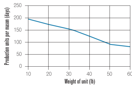
Figure 2. Estimated production rates based on CMU weight. Reprinted with NCMA permission from Kolkoski, R.V., Masonry Estimating. Craftsman Book Company, 1988.
