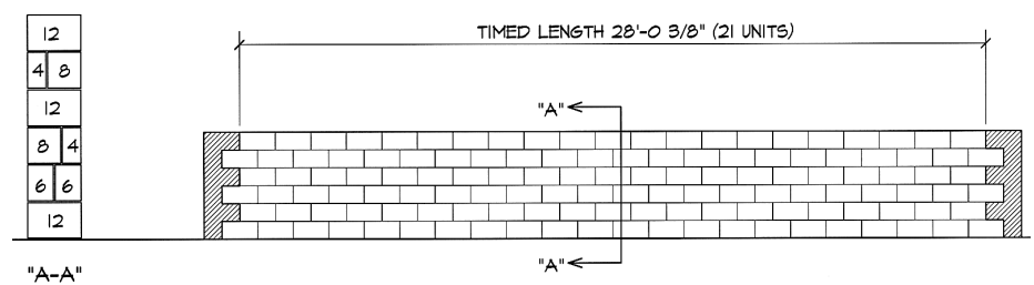
Figure 1. Layout of wall constructed of 16" long CMU.
